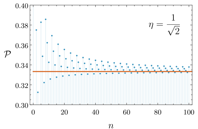
FIG. 6. The probability of an improved recycling scheme with \eta = 1/\sqrt{2} , where we require that the number of photons lost is no more than n/2 when fusing two n -photon states. We see that this probability approaches \sim 1/3 as n \rightarrow \infty .
